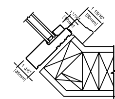
45° WOOD PICTURE 4 9/16\" (116mm)
