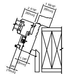
STRAIGHT WALL WOOD CASERMENT 6 9/16" (166 mm) JAMB
