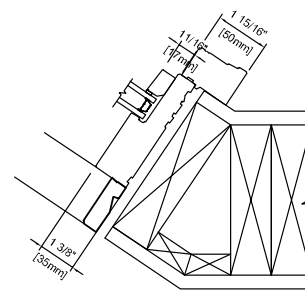
FRAMED WALL WOOD PICTURE 6 9/16\" (166 mm) JAMB
