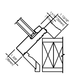
45° WOOD PICTURE 4 9/16" (116mm)
