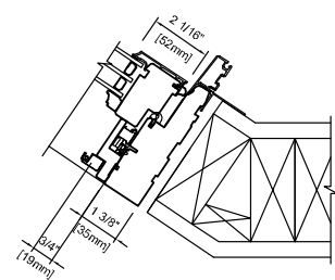
FRAMED WALL METAL CLAD CASEMENT 4 9/16\" (116 mm) JAMB
