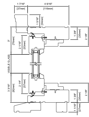
WOOD CASEMENT 4 9/16" (116mm)
