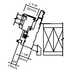
STRAIGHT WALL METAL CLAD CASERMENT 4 9/16" (116 mm) JAMB
