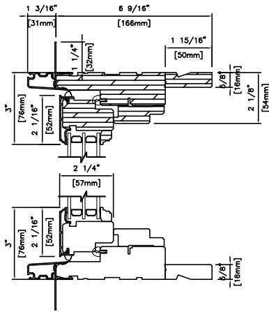
METAL CLAD CASEMENT (TRIPLE GLAZED) 6 9/16" (166mm) ROTOGEAR MOULDINGS
