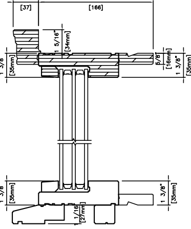
WOOD PICTURE (TRIPLE GLAZED) 6 9/16" (166mm) 2" BRICKMOULD WITH STANDARD SUBSILL
