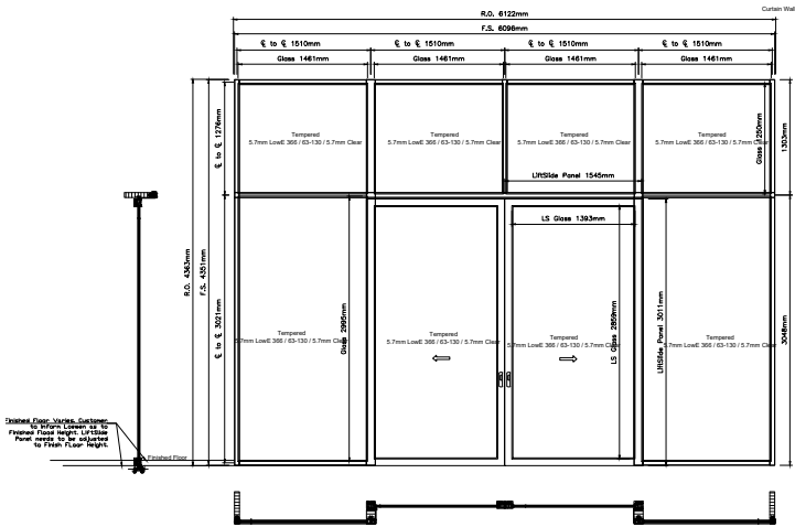
Curtain Wall with LiftSlide Panels OX-XO with Transom
