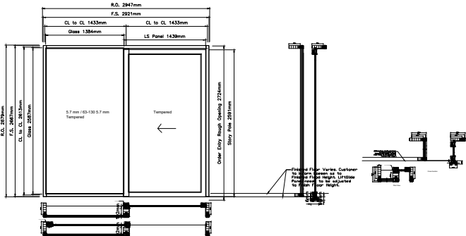
Curtain Wall with LiftSlide Panels OX
