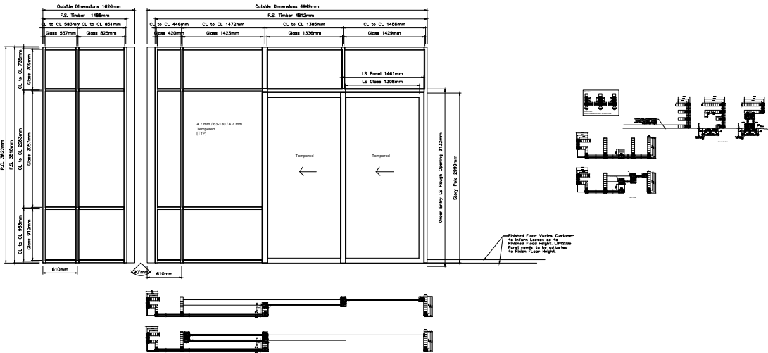
Curtain Wall with LiftSlide Panels Corner with XO & Transom
