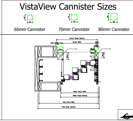
Example using Vista View Screen with 70 mm Canister.
