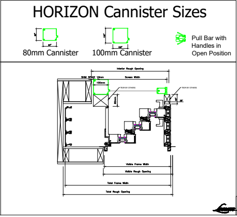
Example using Horizon Screen with 100 mm Canister.
